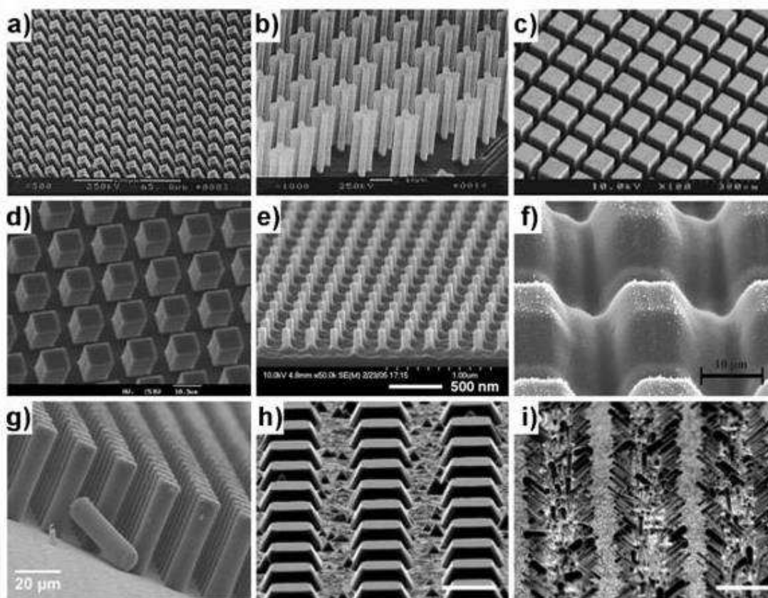
Figure 9. Lithographic surface modification a) photolithographic towers and b) indented square posts, 114 c) diced silicon wafer, 115 d) photolithographic towers, 116 e) silicon nano-towers, 117 f) laser modified SU8 surface, 118 g) SU8 towers, 9 h) silicon islands and i) silicon nano-wires grown on those silicon islands. 119 Figures reprinted with permission from a) b) c) f) h) and i) American Chemical Society, Copyright 2000, 2002, 2006 and 2007, d) Elsevier, Copyright 2006 and e) and g) Institute of Physics, Copyright 2006 and 2004 respectively.
