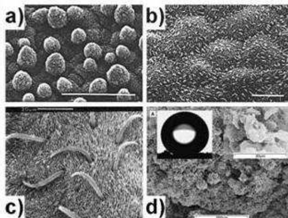
Figure 2. Superhydrophobic surfaces in biology a) Lotus leaf ( Nelumbo Nucifera ), 10 b) Hillock bush leaf, ( Melaleuca hypericifolia ), 10 c) Middle of upper side of a common pond skater ( Gerris lacustris ) 11 and d) the lichen Lecanora Conizaeoides showing high roughness with inset showing water drop WCA 155\pm 4^\circ . 12 Figures reprinted with permission from a) and b) Oxford University Press, Copyright 1997, c) Blackwell Publishing, Copyright 1996 and d) Elsevier, Copyright 2006.
