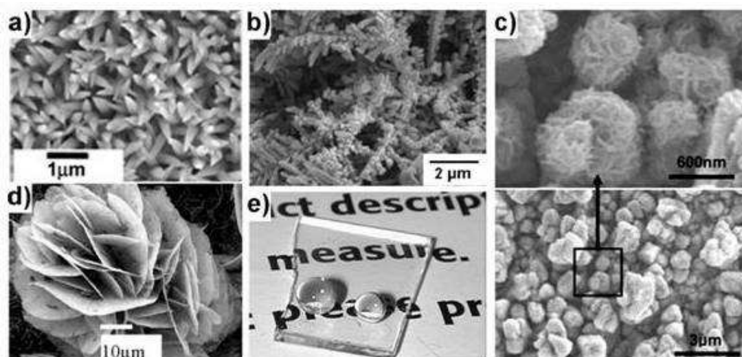
Figure 6. Rough surfaces by crystal growth a) cobalt hydroxide crystalline nano-pins (brucite-type) with diameter of 6.5 nm, 53 b) Silver aggregates deposited on a silicon wafer, 54 c) CuS coated copper oxide; enlargement shows nanostructure, 55 d) Flower-like tin oxide structure, 56 and e) transparent superhydrophobic alumina-silica composite film. 57 Figures reprinted with permission from a) b) American Chemical Society, Copyright 2005 and 2006 respectively, c) and d) The Royal Society of Chemistry, Copyright 2005 and 2004 respectively and e) Institute of Physics, Copyright 2007.
