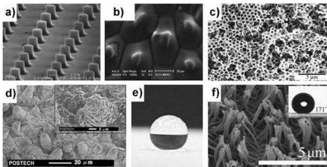
Figure 11. Replica surfaces produced by templating a) micro-posts, 143 b) PMMA replica of Colocasia -like leaf surface, 144 c) a polyvinylidene fluoride inverse opaline structure, 145 d) photoresist replica of lotus leaf by UV-NIL, 127 e) water droplet resting on a polymer hot-press transferred pattern, 146 and f) polymer hairs grown through an AAO template with insert showing water droplet resting on surface. 147 Figures reprinted with permission from a) EDP sciences, Copyright 1999, b) and c) Elsevier, Copyright 2007 and 2006 respectively, d) Institute of Physics, Copyright 2007 and e) and f) American Chemical Society, Copyright 2006.
