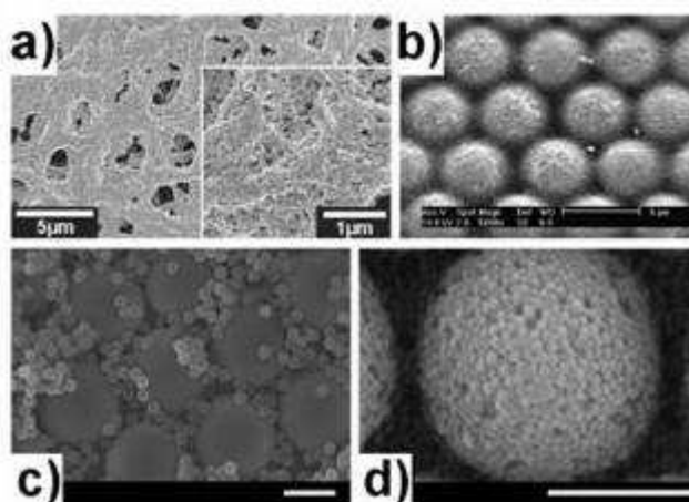
Figure 10. Particle aggregation a) layer-by-layer deposition of \text{TiO}_2 particles on fibres, 26 b) CNT coated polystyrene sphere array, 128 c) silica sphere array with additional smaller sphere aggregates (scale bar 5 \mu\text{m} ) and d) micron sphere array produced from 300 nm particles silica nano-spheres (scale bar 5 \mu\text{m} ). 129 Figures reprinted with permission from a) Institute of Physics, Copyright 2007, b) American Chemical Society, Copyright 2007, c) and d) Elsevier, Copyright 2007.
