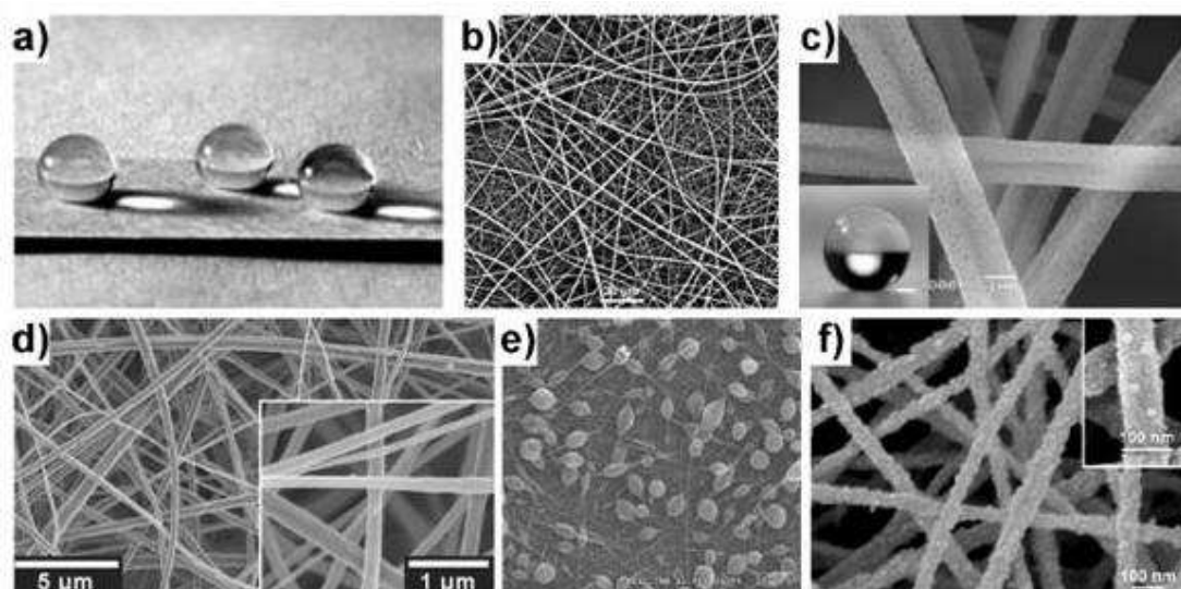
Figure 4. Superhydrophobic fibre surfaces a) water droplets on a block copolymer electrospun fibre mat, 23 b) electrospun fluoropolymer mat, 24 c) porous electrospun fluorinated fibres, 25 d) cellulose acetate fibrous membrane, 26 e) micro-bead connected fibres by electrospinning. 27 Figures reprinted with permission from a) American Chemical Society, Copyright 2005, b) c) and f) Copyright Wiley-VCH Verlag GmbH & Co. KGaA. d) Institute of Physics, Copyright 2007 and e) Elsevier, Copyright 2007.
