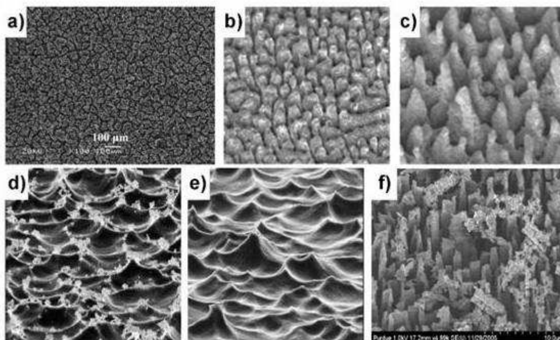
Figure 7. Etching a) roughened aluminium alloy, 79 b) Laser etched silicon surface in SF 6 3.2 kJ/m 2 and c) using 5 kJ/m 2 , 80 d) silicon wafer / photoresist layer over-etched by an inductive SF 6 plasma before cleaning 81 and e) after ultrasonication to remove residual photoresist, and f) submicron pillar structures in p-type silicon after buffered oxide etching. 82 Figures reprinted with permission from a) d) and e) Elsevier, Copyright 2006 and 2005 and b) c) and f) American Chemical Society, Copyright 2006 and 2007.
