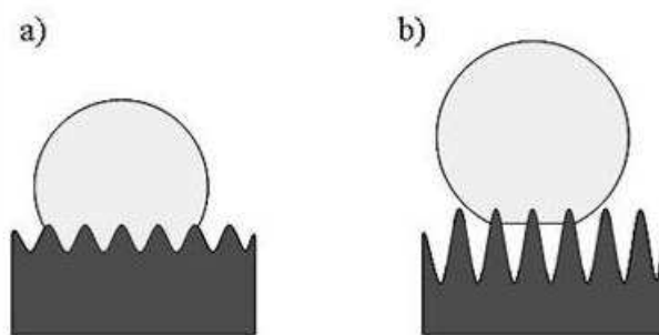
Figure 1. Wetting states a) Wenzel and b) Cassie-Baxter models.
