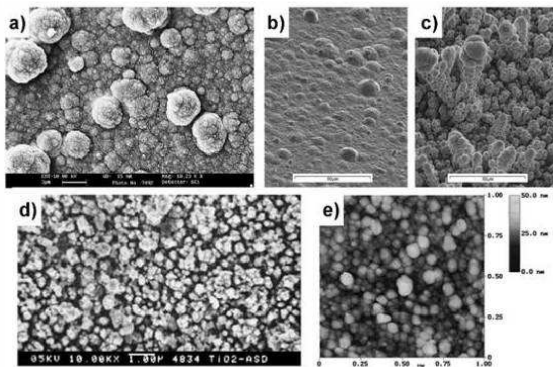
Figure 8. Diffusion limited growth on surfaces a) plasma deposited Teflon structures, 96 b) electrochemically deposited copper at 100 mA cm -2 and c) 200 mA cm -2 , 8 d) an electrodeposited amorphous TiO 2 thin film, 97 and e) HMDS plasma deposited polymer. 98 Figures reprinted with permission from a) d) and e) Elsevier, Copyright 2007, 2005 and 2001 respectively and b) and c) American Chemical Society, Copyright 2005.
