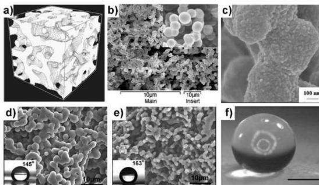
Figure 5. Examples of phase separation, a) model of a bicontinuous structure, 39 b) sol-gel foam produced using acetone as co-solvent, 40 c) super-hydrophobic PVC film, 41 d) and e) phase separated block copolymer films, 42 f) water droplet on an organic xerogel (scale bar 1 mm) 43 Figures reprinted with permission from a) American Physical Society, Copyright 2001, b) and c) from Elsevier, Copyright 2007 and 2006 respectively, d) and e) from American Chemical Society, Copyright 2005 and f) The Royal Society of Chemistry, Copyright 2006.
