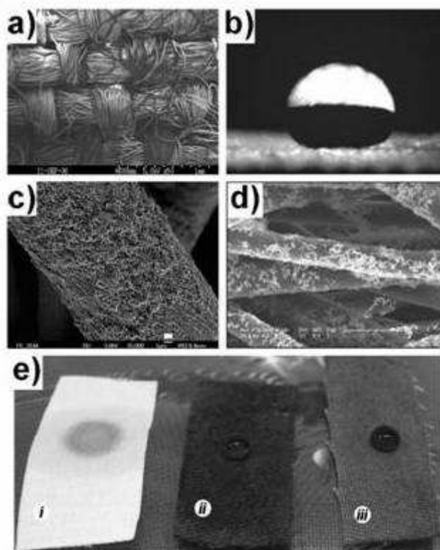
Figure 3. Woven superhydrophobic surfaces a) multifilament woven fabric, 15 b) droplet resting on surface shown in a), c) CNT treated cotton fibre, 16 d) cloth surface impregnated with gold particles, 17 and e) water droplets on 16 i) untreated woven cotton sheet, ii) CNT treated woven cotton sheet shown in c) and iii) poly(butyl acrylate)-CNT treated woven cotton sheet. Figures reprinted with permission from a) and b) American Chemical Society, Copyright 2007, c) d) and e) The Royal Society of Chemistry, Copyright 2007.
